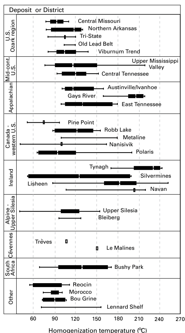
Figure 8. Summary of homogenization temperatures for sphalerite for selected Mississippi Valley-Type deposits based on fluid inclusion studies (from Leach and others, 2005).
