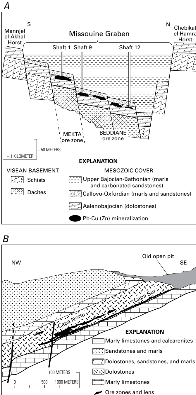
Figure 6. Geology and mineralization in select Mississippi Valley-Type (MVT) deposits. (A) Generalized section showing piano keylike horst/graben structure of the Toussit-Bou Beker mining district, Morocco (from Bouabdella and others, 1996). (B) Cross section through the central part of the Reocin deposit, Spain, showing the relation of the ore lenses and the host dolostones (from Leach and others, 2005; modified from Velasco and others, 2003).
