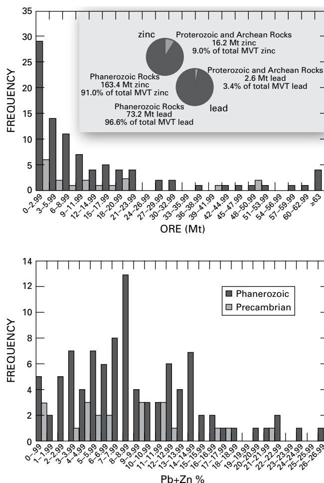
Figure 2. Comparison of metal content and size of Precambrian and Phanerozoic Mississippi Valley-Type (MVT) deposits. Phanerozoic MVT deposits greatly outnumber and contain a greater quantity of metal than Precambrian deposits.
